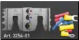
DIN 0.5-1.0 / 1.5-2.5 / 4-6 mm² AWG 22-18 / 16-14 / 12-10
